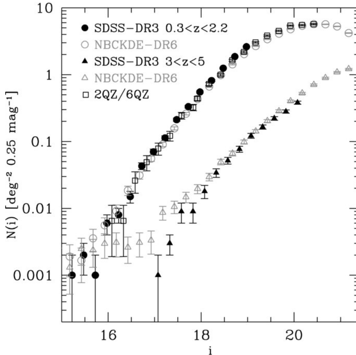
Figure 18. from Efficient Photometric Selection of Quasars from the Sloan Digital Sky Survey. II. 1,000,000 Quasars from Data Release 6 RICHARDS ET AL. 2009 ApJS 180 67 doi:10.1088/0067-0049/180/1/67 https://dx.doi.org/10.1088/0067-0049/180/1/67 © 2009. The American Astronomical Society. All rights reserved.
