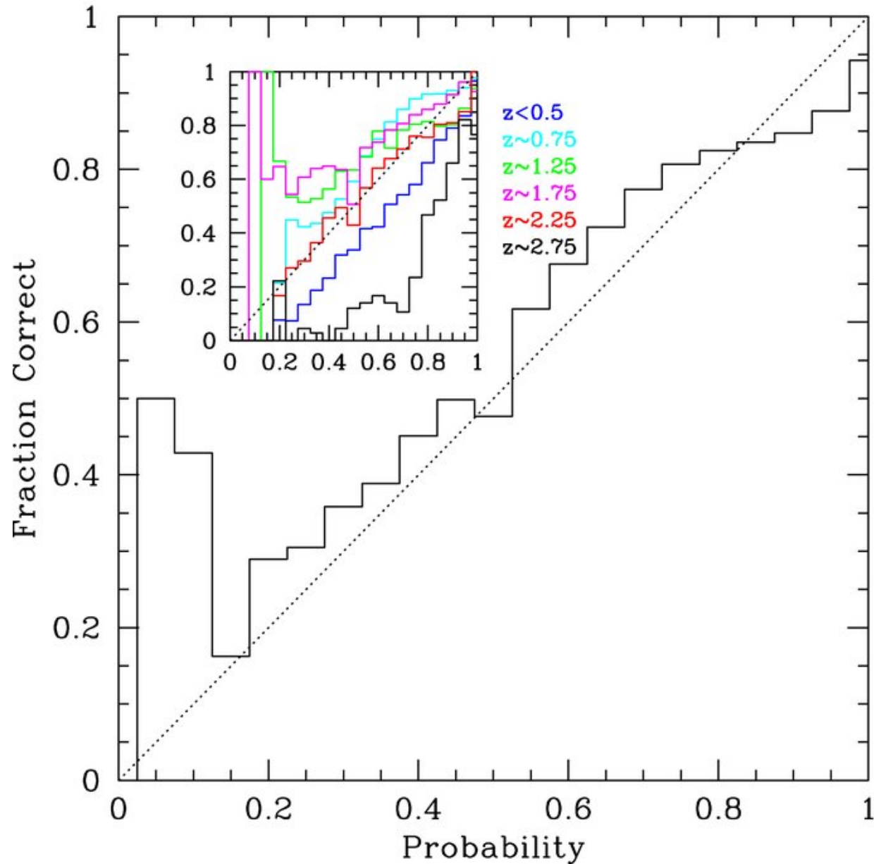
Figure 15. from Efficient Photometric Selection of Quasars from the Sloan Digital Sky Survey. II. 1,000,000 Quasars from Data Release 6 RICHARDS ET AL. 2009 ApJS 180 67 doi:10.1088/0067-0049/180/1/67 https://dx.doi.org/10.1088/0067-0049/180/1/67 © 2009. The American Astronomical Society. All rights reserved.
