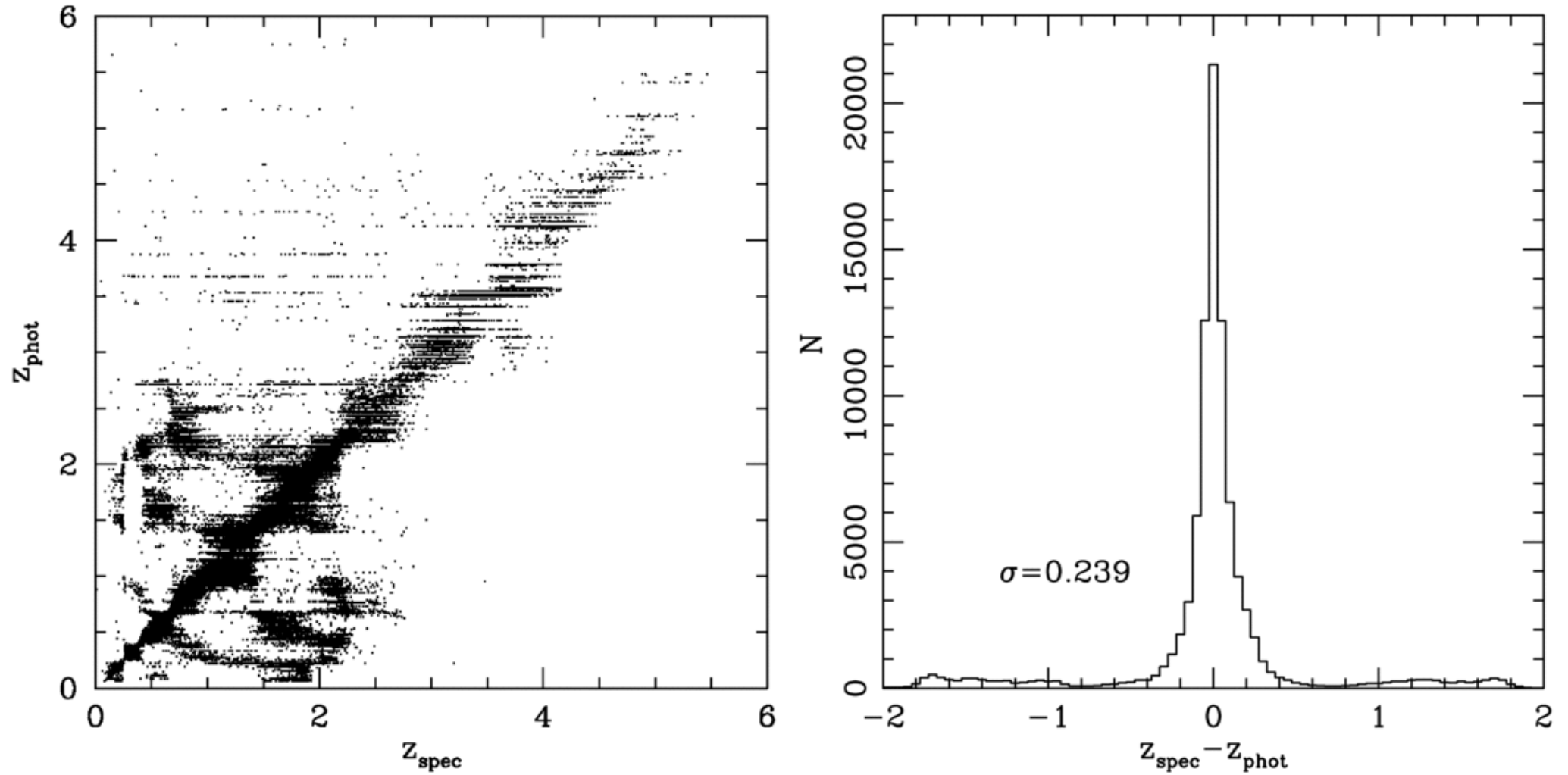
Figure 13. from Efficient Photometric Selection of Quasars from the Sloan Digital Sky Survey. II. 1,000,000 Quasars from Data Release 6 RICHARDS ET AL. 2009 ApJS 180 67 doi:10.1088/0067-0049/180/1/67 https://dx.doi.org/10.1088/0067-0049/180/1/67 © 2009. The American Astronomical Society. All rights reserved.
