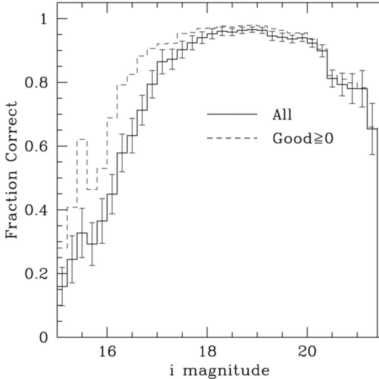
Figure 11. from Efficient Photometric Selection of Quasars from the Sloan Digital Sky Survey. II. 1,000,000 Quasars from Data Release 6 RICHARDS ET AL. 2009 ApJS 180 67 doi:10.1088/0067-0049/180/1/67 https://dx.doi.org/10.1088/0067-0049/180/1/67 © 2009. The American Astronomical Society. All rights reserved.
