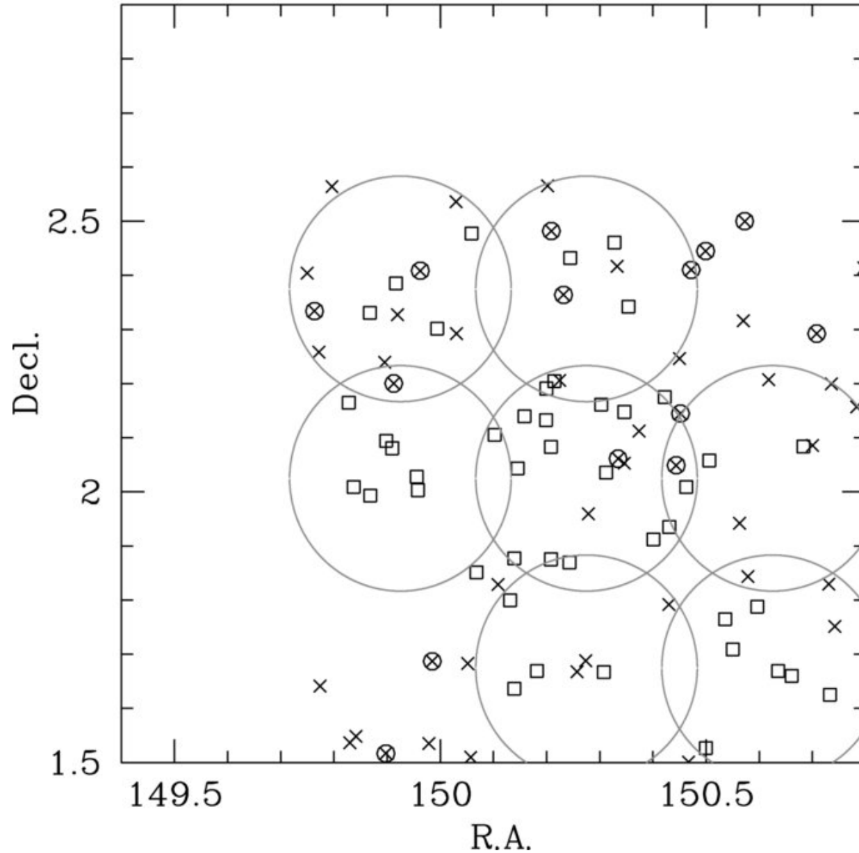
Figure 10. from Efficient Photometric Selection of Quasars from the Sloan Digital Sky Survey. II. 1,000,000 Quasars from Data Release 6 RICHARDS ET AL. 2009 ApJS 180 67 doi:10.1088/0067-0049/180/1/67 https://dx.doi.org/10.1088/0067-0049/180/1/67 © 2009. The American Astronomical Society. All rights reserved.
