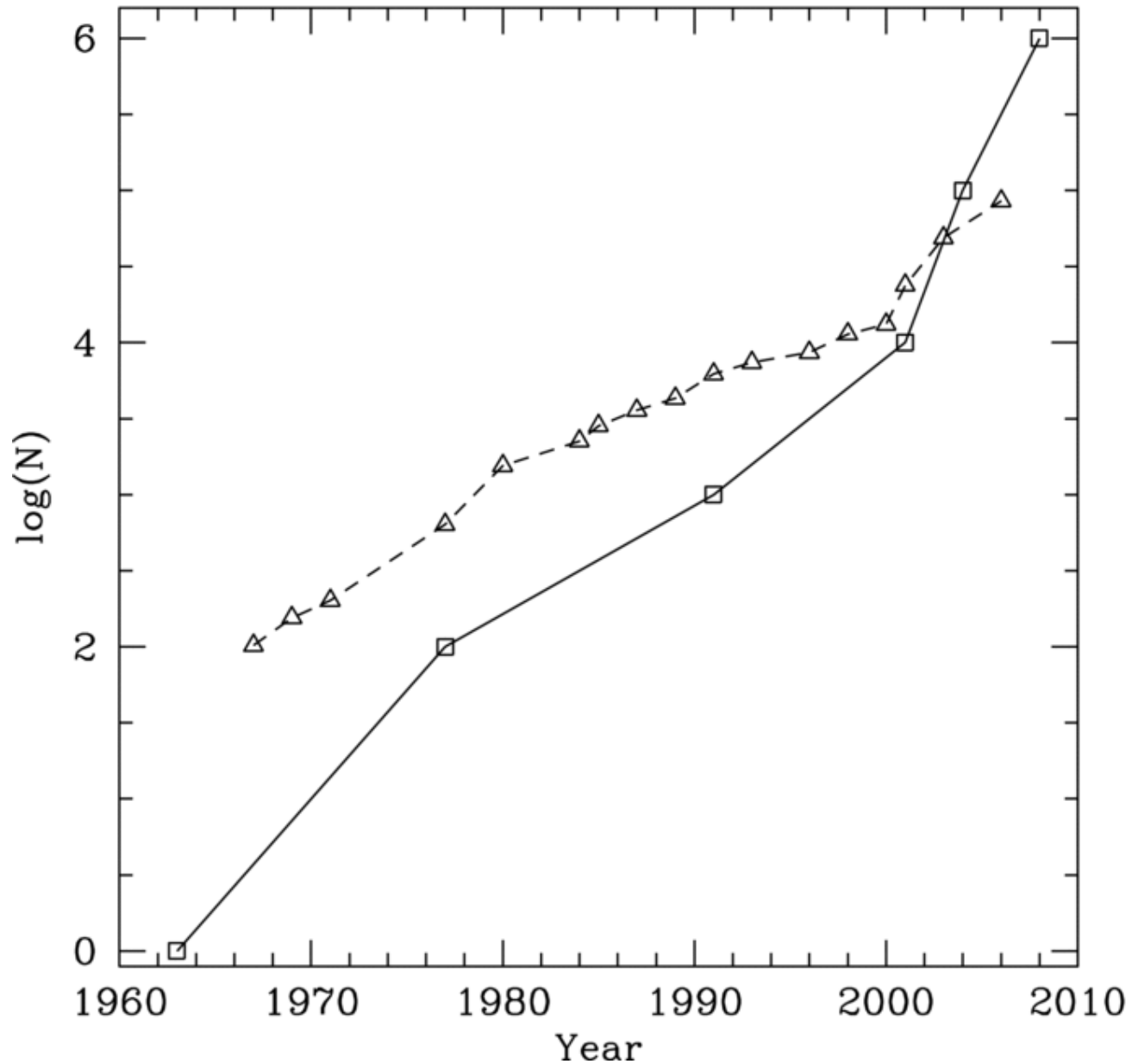
Figure 1. from Efficient Photometric Selection of Quasars from the Sloan Digital Sky Survey. II. 1,000,000 Quasars from Data Release 6 RICHARDS ET AL. 2009 ApJS 180 67 doi:10.1088/0067-0049/180/1/67 https://dx.doi.org/10.1088/0067-0049/180/1/67 © 2009. The American Astronomical Society. All rights reserved.
