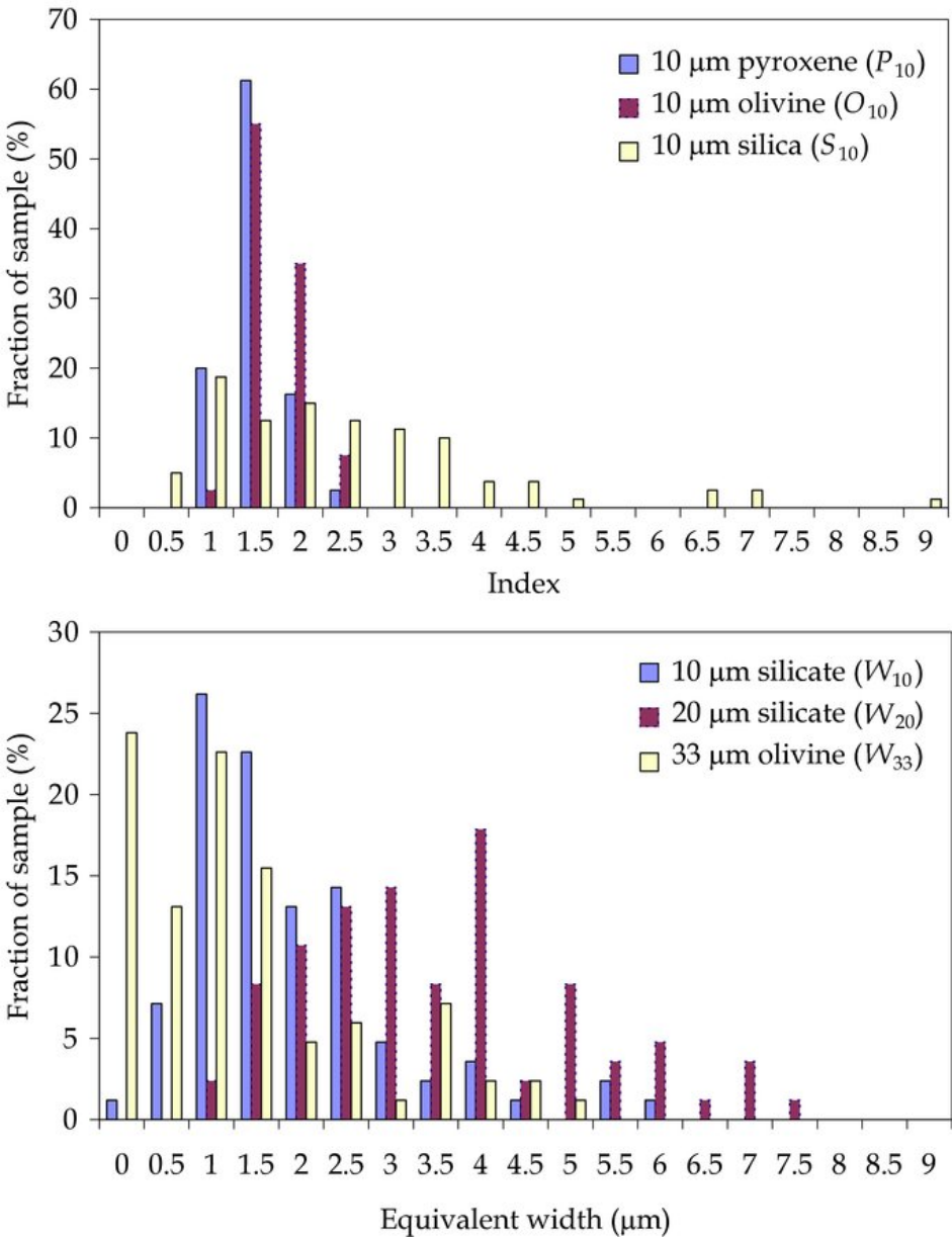
Figure 5. from Crystalline Silicates and Dust Processing in the Protoplanetary Disks of the Taurus Young Cluster WATSON ET AL. 2009 ApJS 180 84 doi:10.1088/0067-0049/180/1/84 https://dx.doi.org/10.1088/0067-0049/180/1/84 © 2009. The American Astronomical Society. All rights reserved.
