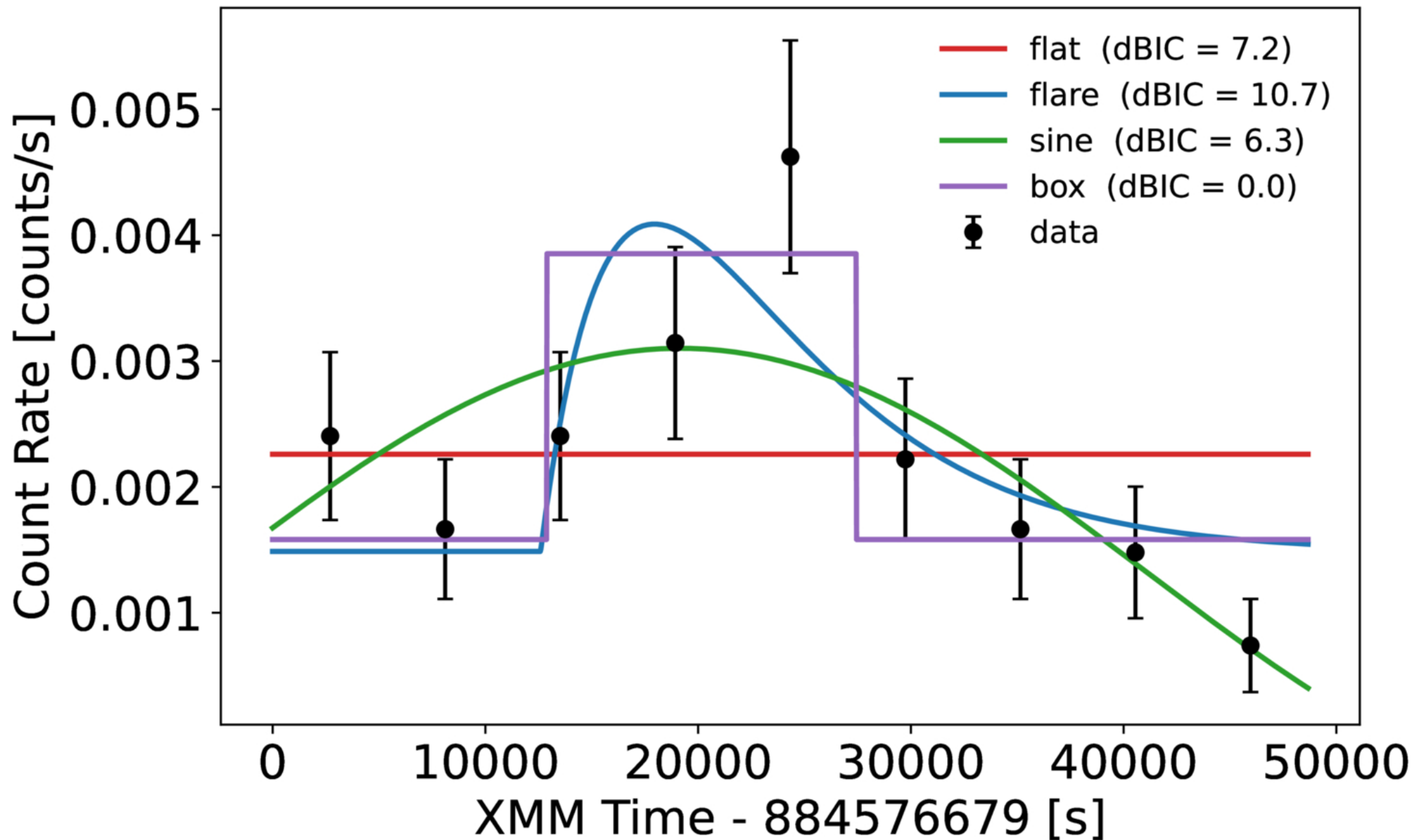
Figure A5. from Collin Cherubim et al 2026 Astrophys. J. Lett. 1011 doi:10.3847/2041-8213/aeb41e https://dx.doi.org/10.3847/2041-8213/aeb41e © 2026. The Author(s). Published by the American Astronomical Society.
