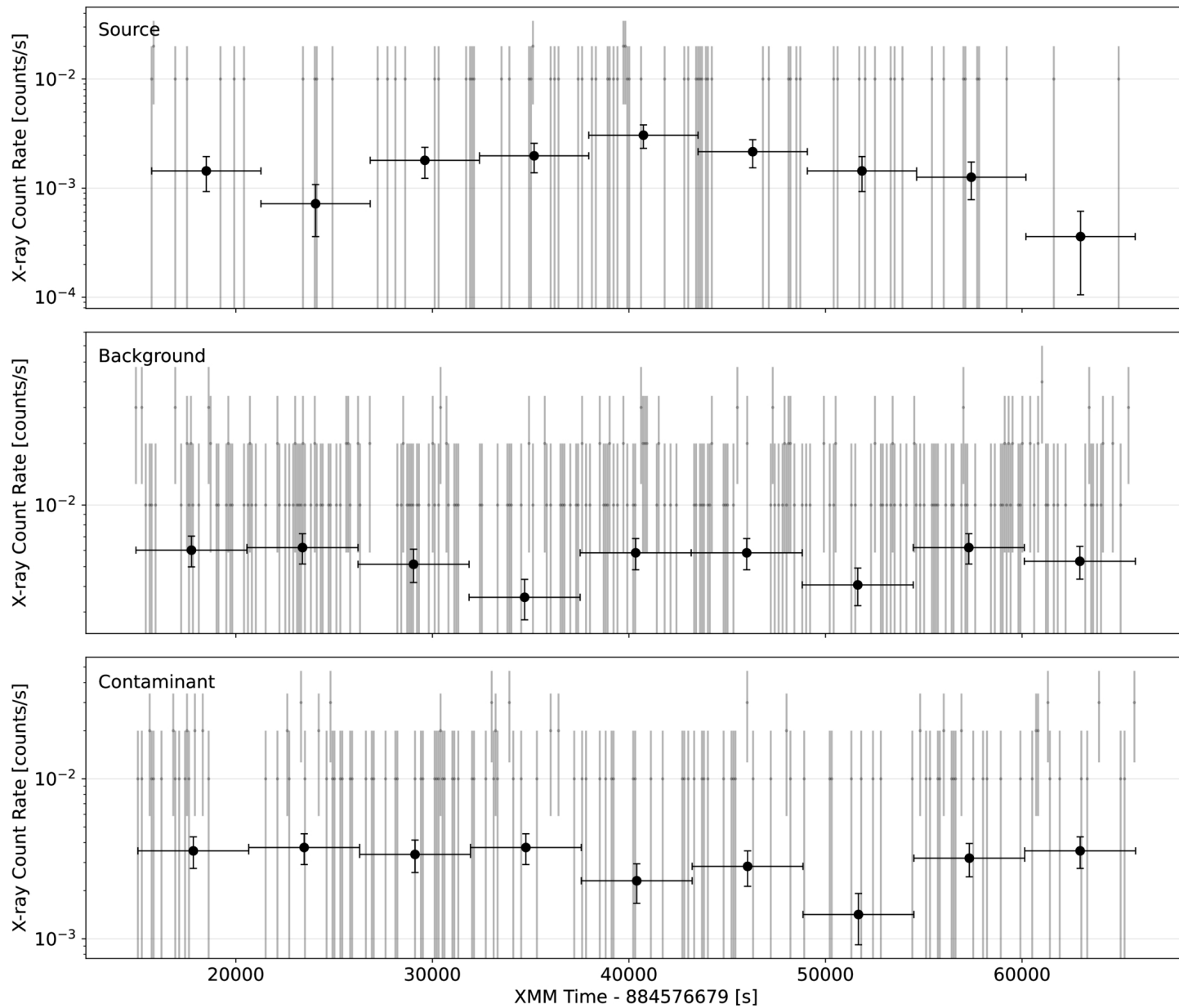
Figure A3. from Collin Cherubim et al 2026 Astrophys. J. Lett. 1011 doi:10.3847/2041-8213/aeb41e https://dx.doi.org/10.3847/2041-8213/aeb41e © 2026. The Author(s). Published by the American Astronomical Society.
