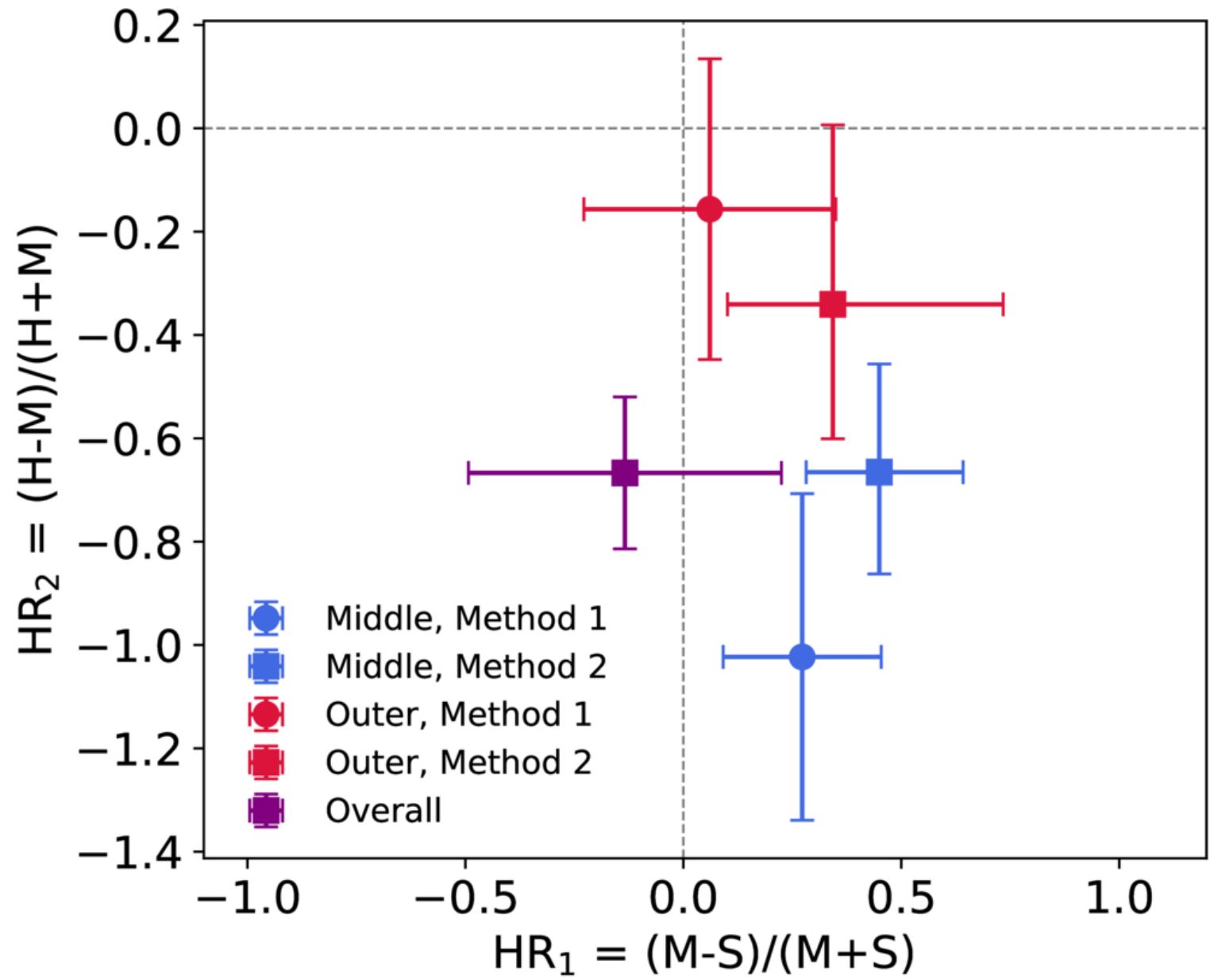
Figure A7. from Collin Cherubim et al 2026 Astrophys. J. Lett. 1011 doi:10.3847/2041-8213/aeb41e https://dx.doi.org/10.3847/2041-8213/aeb41e © 2026. The Author(s). Published by the American Astronomical Society.
