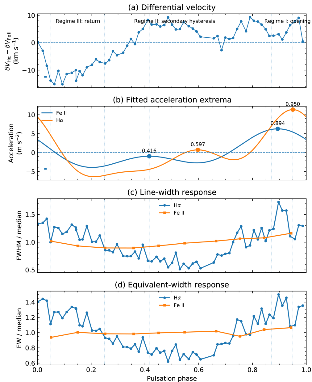
Figure 3. from Merieme Chadid et al 2026 Astrophys. J. Lett. 1010 doi:10.3847/2041-8213/aeace1 https://dx.doi.org/10.3847/2041-8213/aeace1 © 2026. The Author(s). Published by the American Astronomical Society.
