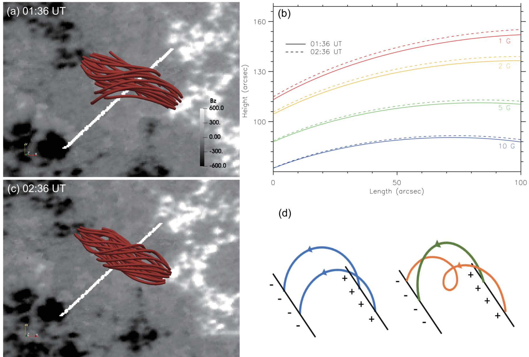
Figure 5. from Ye Qiu et al 2026 Astrophys. J. Lett. 1010 doi:10.3847/2041-8213/aeacda https://dx.doi.org/10.3847/2041-8213/aeacda © 2026. The Author(s). Published by the American Astronomical Society.
