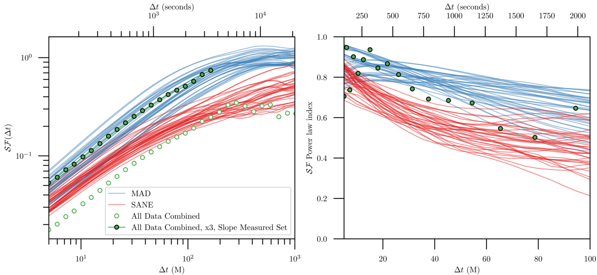
Figure 5. from Daniel C. M. Palumbo et al 2026 Astrophys. J. Lett. 1010 doi:10.3847/2041-8213/aeacd0 https://dx.doi.org/10.3847/2041-8213/aeacd0 © 2026. The Author(s). Published by the American Astronomical Society.
