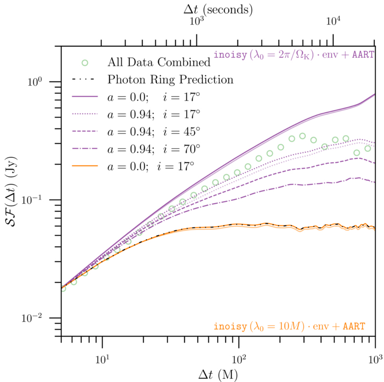
Figure 4. from Daniel C. M. Palumbo et al 2026 Astrophys. J. Lett. 1010 doi:10.3847/2041-8213/aeacd0 https://dx.doi.org/10.3847/2041-8213/aeacd0 © 2026. The Author(s). Published by the American Astronomical Society.
