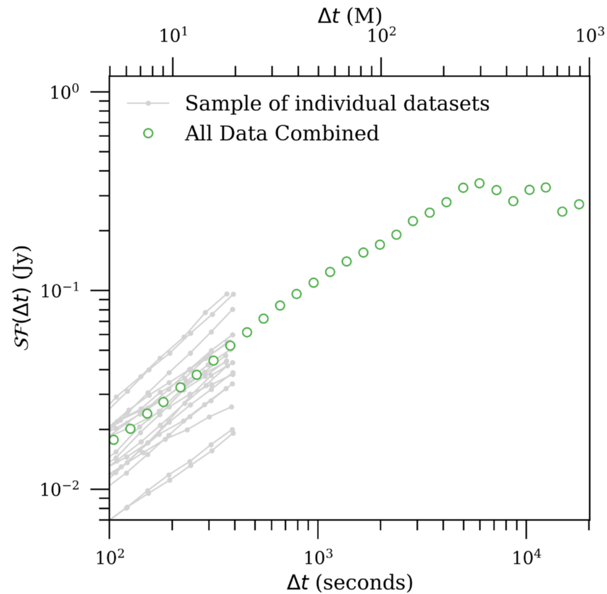
Figure 2. from Daniel C. M. Palumbo et al 2026 Astrophys. J. Lett. 1010 doi:10.3847/2041-8213/aeacd0 https://dx.doi.org/10.3847/2041-8213/aeacd0 © 2026. The Author(s). Published by the American Astronomical Society.
