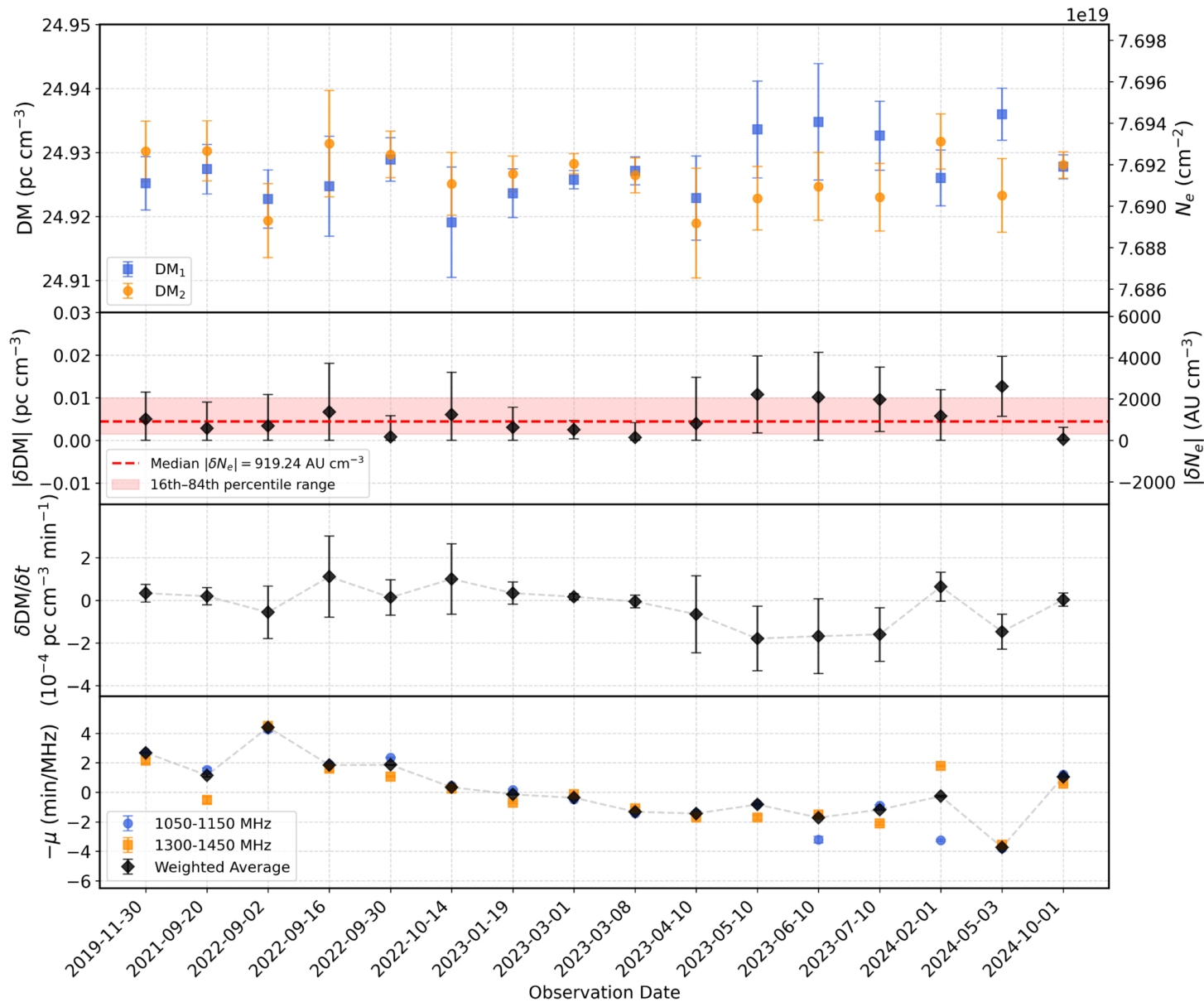
Figure 2. from Qiuyi He et al 2026 Astrophys. J. Lett. 1010 doi:10.3847/2041-8213/aeacbd https://dx.doi.org/10.3847/2041-8213/aeacbd © 2026. The Author(s). Published by the American Astronomical Society.
