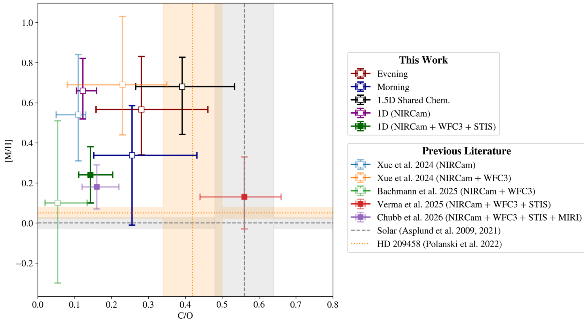
Figure A4. from Cathal Maguire et al 2026 Astrophys. J. Lett. 1010 doi:10.3847/2041-8213/aeac49 https://dx.doi.org/10.3847/2041-8213/aeac49 © 2026. The Author(s). Published by the American Astronomical Society.
