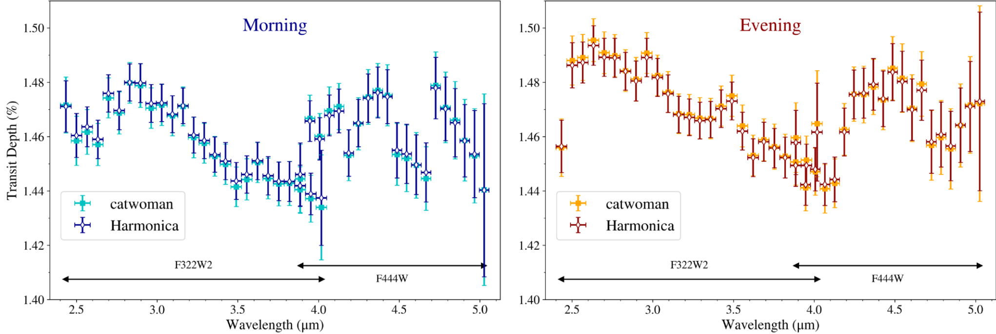
Figure 2. from Cathal Maguire et al 2026 Astrophys. J. Lett. 1010 doi:10.3847/2041-8213/aeac49 https://dx.doi.org/10.3847/2041-8213/aeac49 © 2026. The Author(s). Published by the American Astronomical Society.
