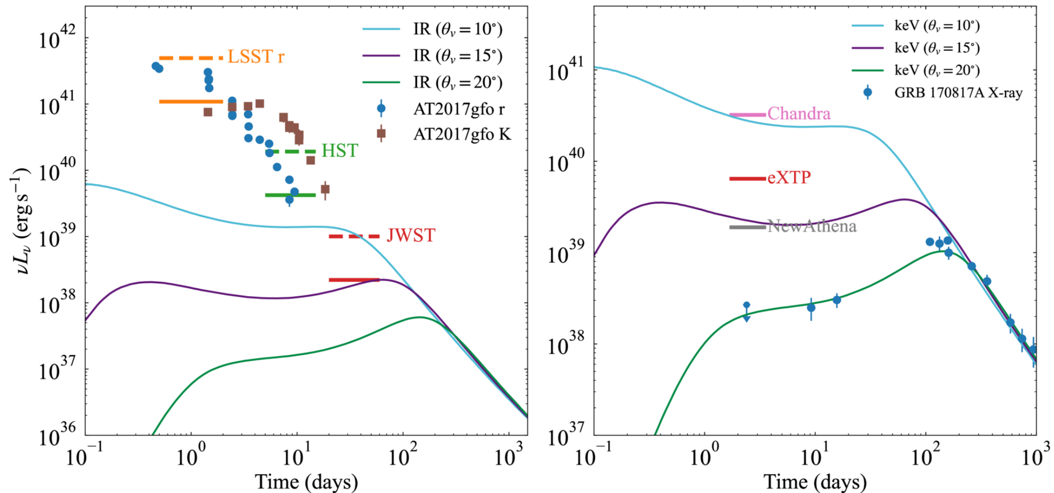
Figure 9. from Jian-He Zheng and Wenbin Lu 2026 Astrophys. J. Lett. 1010 doi:10.3847/2041-8213/aeac25 https://dx.doi.org/10.3847/2041-8213/aeac25 © 2026. The Author(s). Published by the American Astronomical Society.
