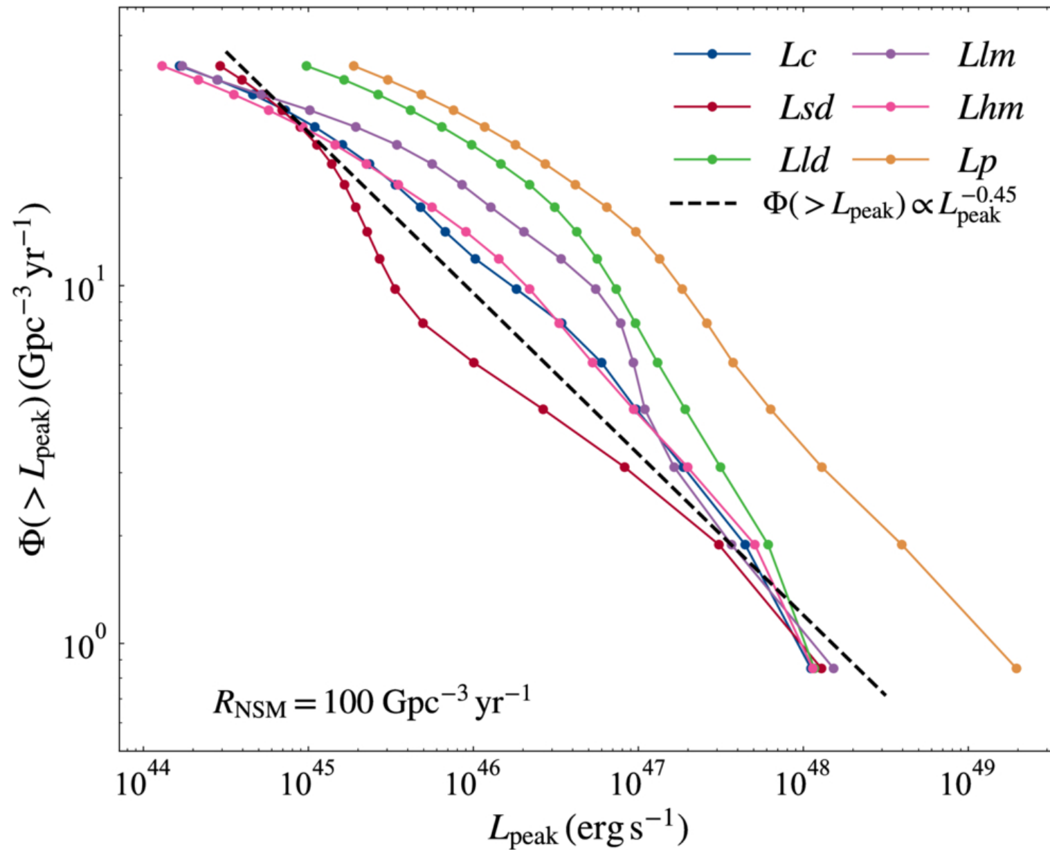
Figure 8. from Jian-He Zheng and Wenbin Lu 2026 Astrophys. J. Lett. 1010 doi:10.3847/2041-8213/aeac25 https://dx.doi.org/10.3847/2041-8213/aeac25 © 2026. The Author(s). Published by the American Astronomical Society.
