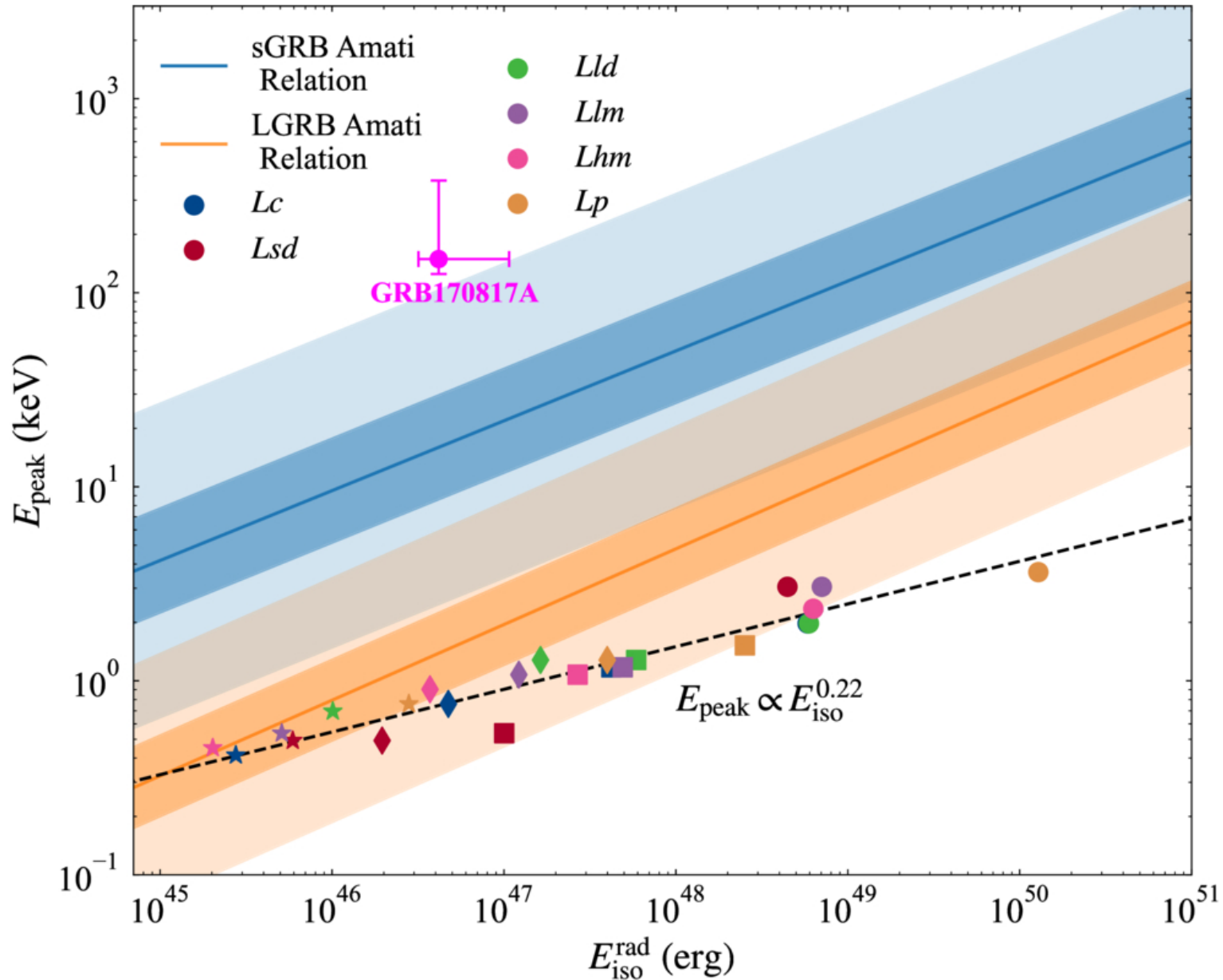
Figure 7. from Jian-He Zheng and Wenbin Lu 2026 Astrophys. J. Lett. 1010 doi:10.3847/2041-8213/aeac25 https://dx.doi.org/10.3847/2041-8213/aeac25 © 2026. The Author(s). Published by the American Astronomical Society.
