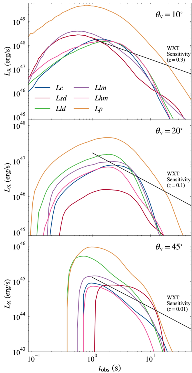
Figure 4. from Jian-He Zheng and Wenbin Lu 2026 Astrophys. J. Lett. 1010 doi:10.3847/2041-8213/aeac25 https://dx.doi.org/10.3847/2041-8213/aeac25 © 2026. The Author(s). Published by the American Astronomical Society.
