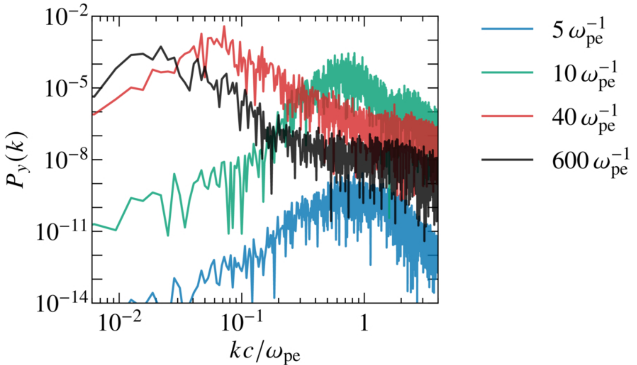
Figure 3. from Kazuki Kamiido and Yutaka Ohira 2026 Astrophys. J. Lett. 1010 doi:10.3847/2041-8213/aeaba2 https://dx.doi.org/10.3847/2041-8213/aeaba2 © 2026. The Author(s). Published by the American Astronomical Society.
