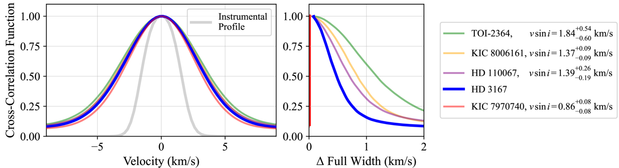
Figure 1. from Joshua N. Winn et al 2026 Astrophys. J. Lett. 1010 doi:10.3847/2041-8213/aeab9d https://dx.doi.org/10.3847/2041-8213/aeab9d © 2026. The Author(s). Published by the American Astronomical Society.
