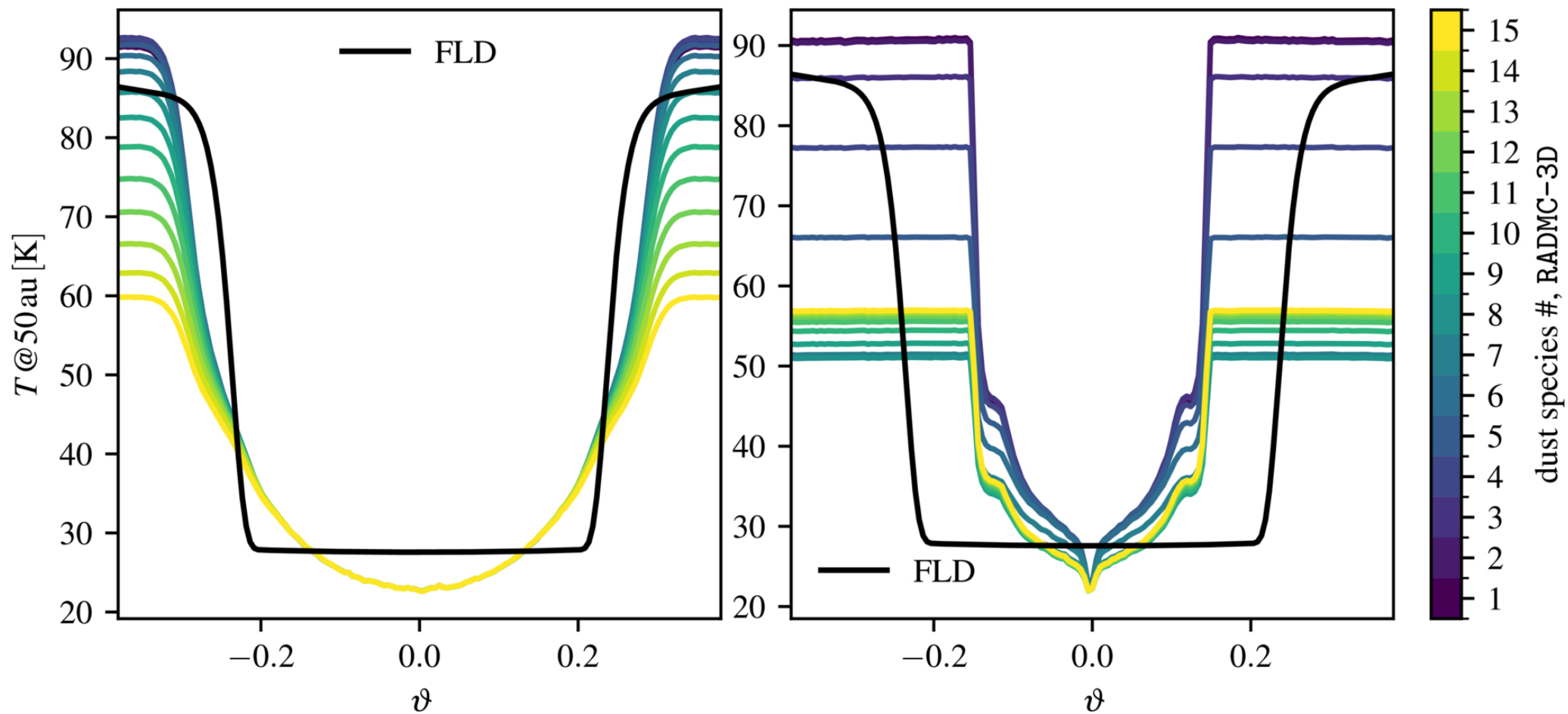
Figure C1. from Thomas Pfeil et al 2026 Astrophys. J. Lett. 1010 doi:10.3847/2041-8213/aeab96 https://dx.doi.org/10.3847/2041-8213/aeab96 © 2026. The Author(s). Published by the American Astronomical Society.
