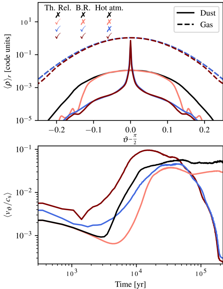
Figure 3. from Thomas Pfeil et al 2026 Astrophys. J. Lett. 1010 doi:10.3847/2041-8213/aeab96 https://dx.doi.org/10.3847/2041-8213/aeab96 © 2026. The Author(s). Published by the American Astronomical Society.
