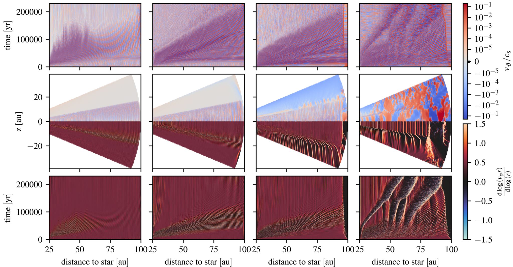
a: Dust-gas thermal coupling Passive dust fluid Vertically Isothermal
