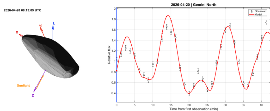
Figure B1. from Xiaoyu Sun et al 2026 Astrophys. J. Lett. 1010 doi:10.3847/2041-8213/aeaa5b https://dx.doi.org/10.3847/2041-8213/aeaa5b © 2026. The Author(s). Published by the American Astronomical Society.
