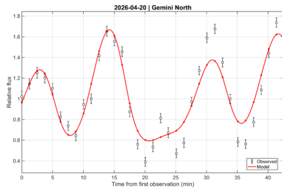
Figure A2. from Xiaoyu Sun et al 2026 Astrophys. J. Lett. 1010 doi:10.3847/2041-8213/aeaa5b https://dx.doi.org/10.3847/2041-8213/aeaa5b © 2026. The Author(s). Published by the American Astronomical Society.
