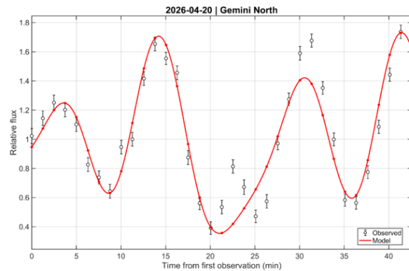
Figure A1. from Xiaoyu Sun et al 2026 Astrophys. J. Lett. 1010 doi:10.3847/2041-8213/aeaa5b https://dx.doi.org/10.3847/2041-8213/aeaa5b © 2026. The Author(s). Published by the American Astronomical Society.
