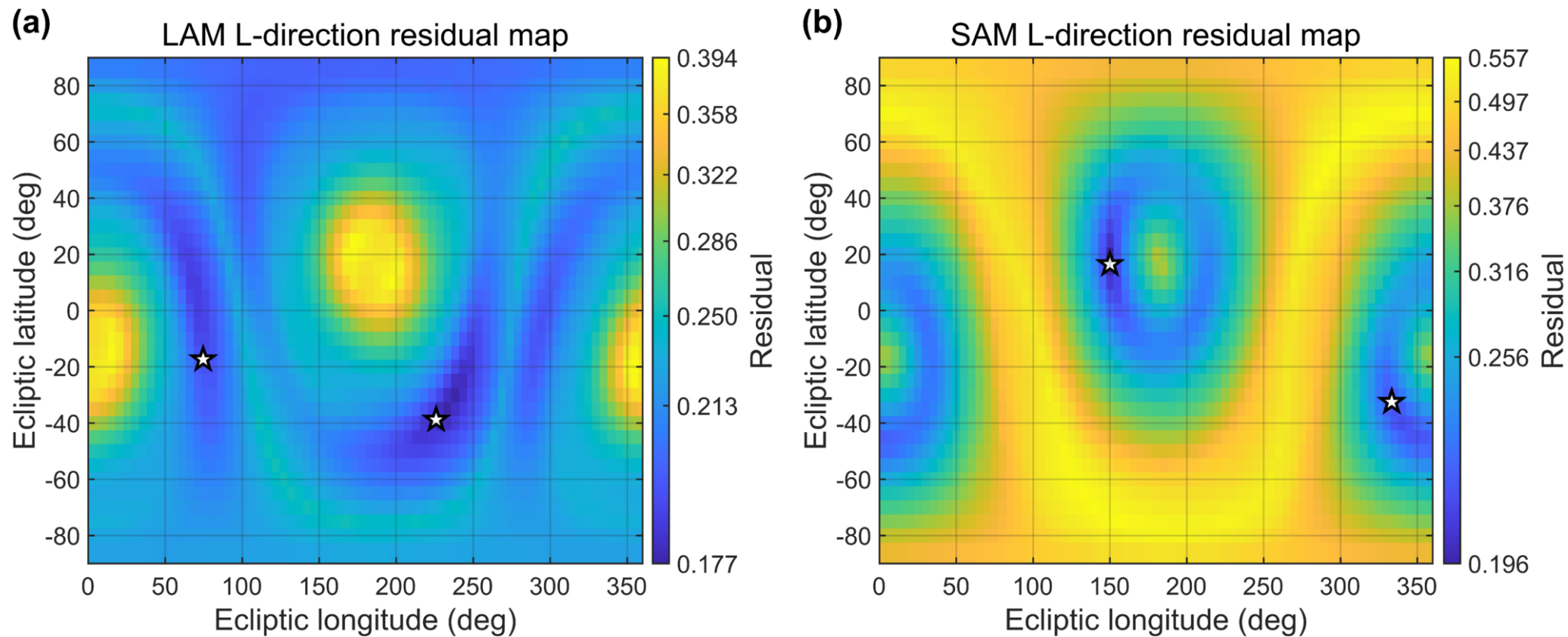
Figure 3. from Xiaoyu Sun et al 2026 Astrophys. J. Lett. 1010 doi:10.3847/2041-8213/aeaa5b https://dx.doi.org/10.3847/2041-8213/aeaa5b © 2026. The Author(s). Published by the American Astronomical Society.
