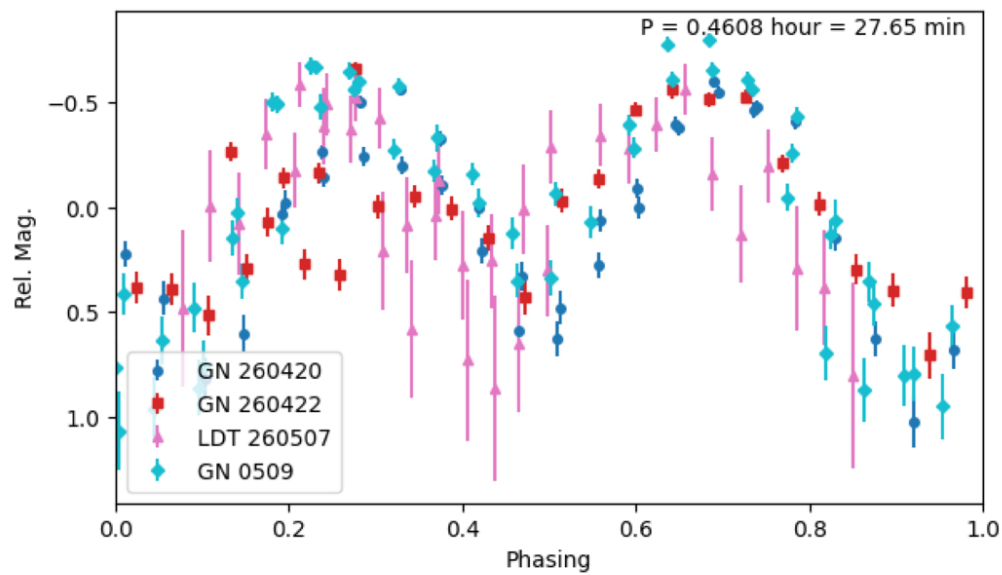
Figure 2. from Xiaoyu Sun et al 2026 Astrophys. J. Lett. 1010 doi:10.3847/2041-8213/aeaa5b https://dx.doi.org/10.3847/2041-8213/aeaa5b © 2026. The Author(s). Published by the American Astronomical Society.
