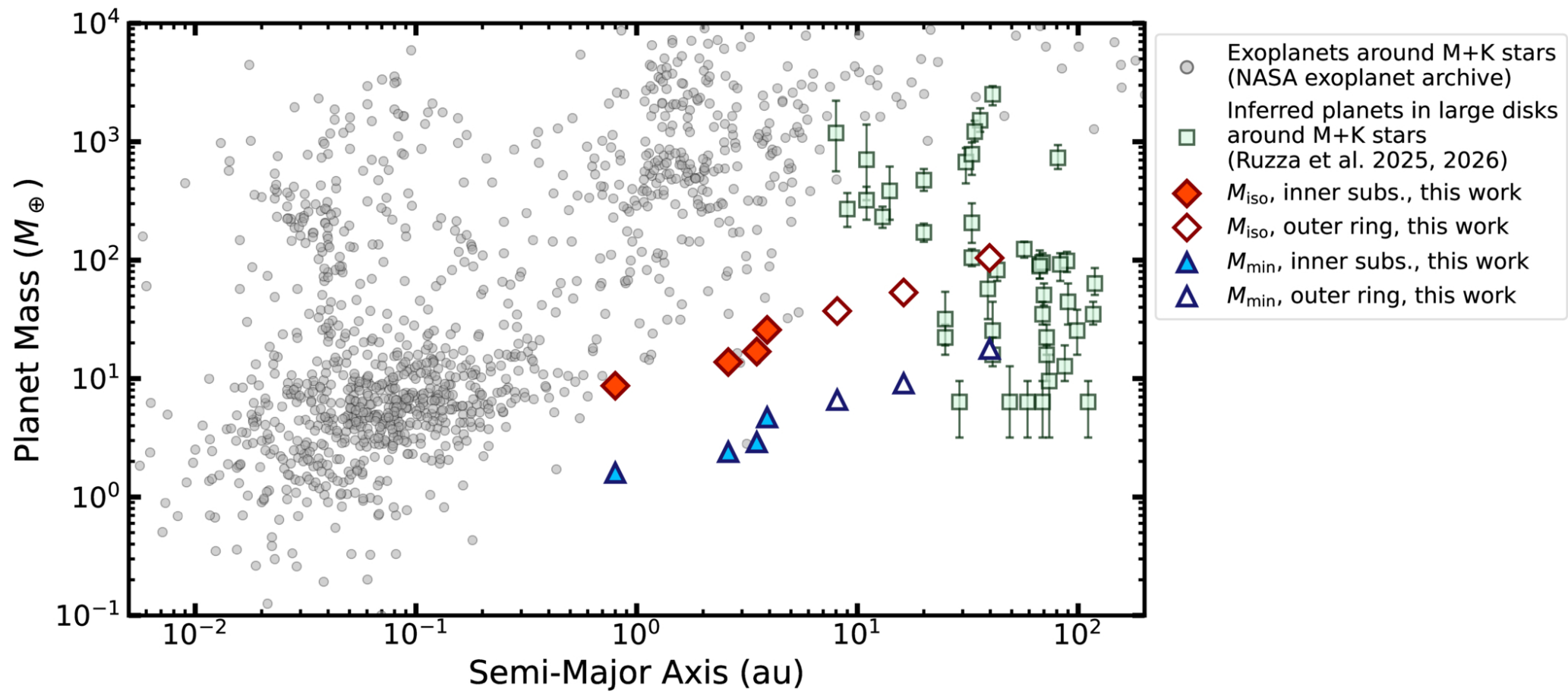
Figure 9. from Pietro Curone et al 2026 Astrophys. J. Lett. 1010 doi:10.3847/2041-8213/aeaa3c https://dx.doi.org/10.3847/2041-8213/aeaa3c © 2026. The Author(s). Published by the American Astronomical Society.
