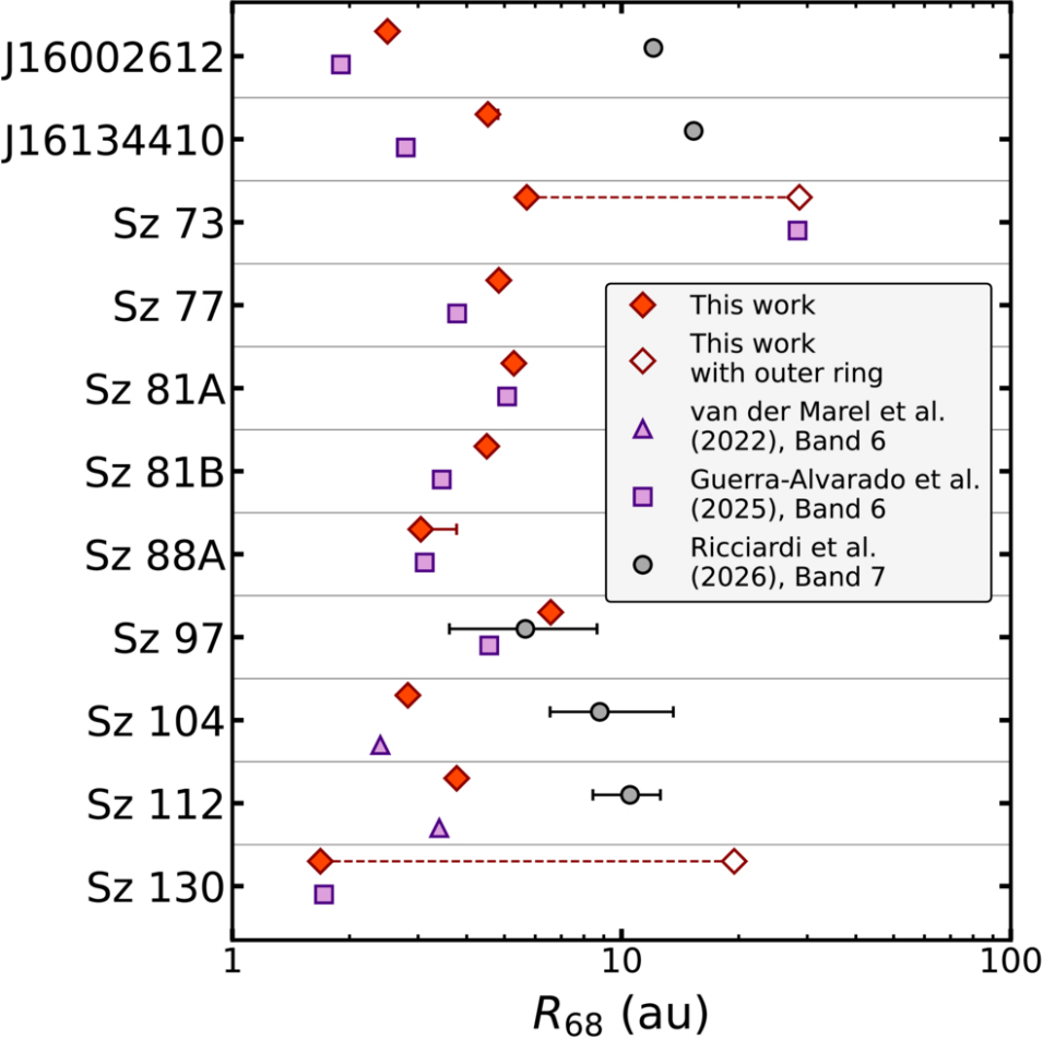
Figure 8. from Pietro Curone et al 2026 Astrophys. J. Lett. 1010 doi:10.3847/2041-8213/aeaa3c https://dx.doi.org/10.3847/2041-8213/aeaa3c © 2026. The Author(s). Published by the American Astronomical Society.
