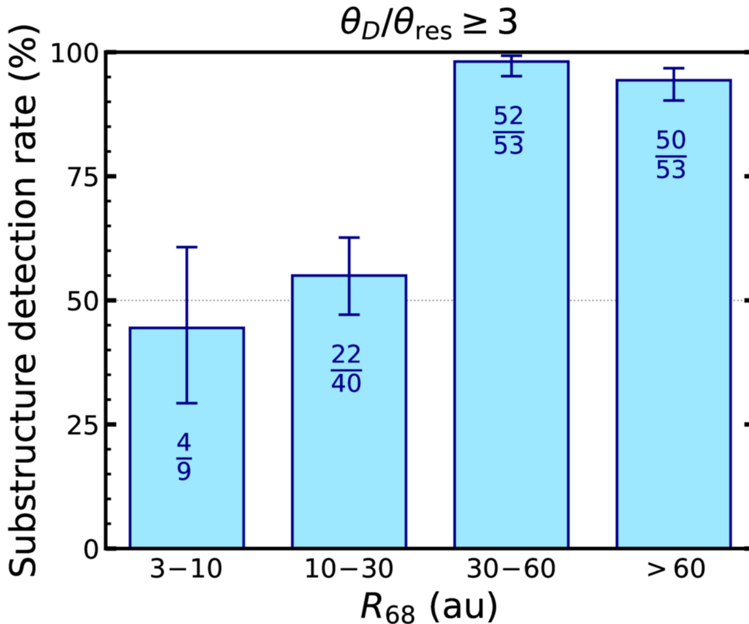
Figure 7. from Pietro Curone et al 2026 Astrophys. J. Lett. 1010 doi:10.3847/2041-8213/aeaa3c https://dx.doi.org/10.3847/2041-8213/aeaa3c © 2026. The Author(s). Published by the American Astronomical Society.
