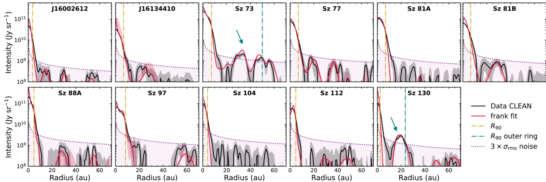
Figure 6. from Pietro Curone et al 2026 Astrophys. J. Lett. 1010 doi:10.3847/2041-8213/aeaa3c https://dx.doi.org/10.3847/2041-8213/aeaa3c © 2026. The Author(s). Published by the American Astronomical Society.
