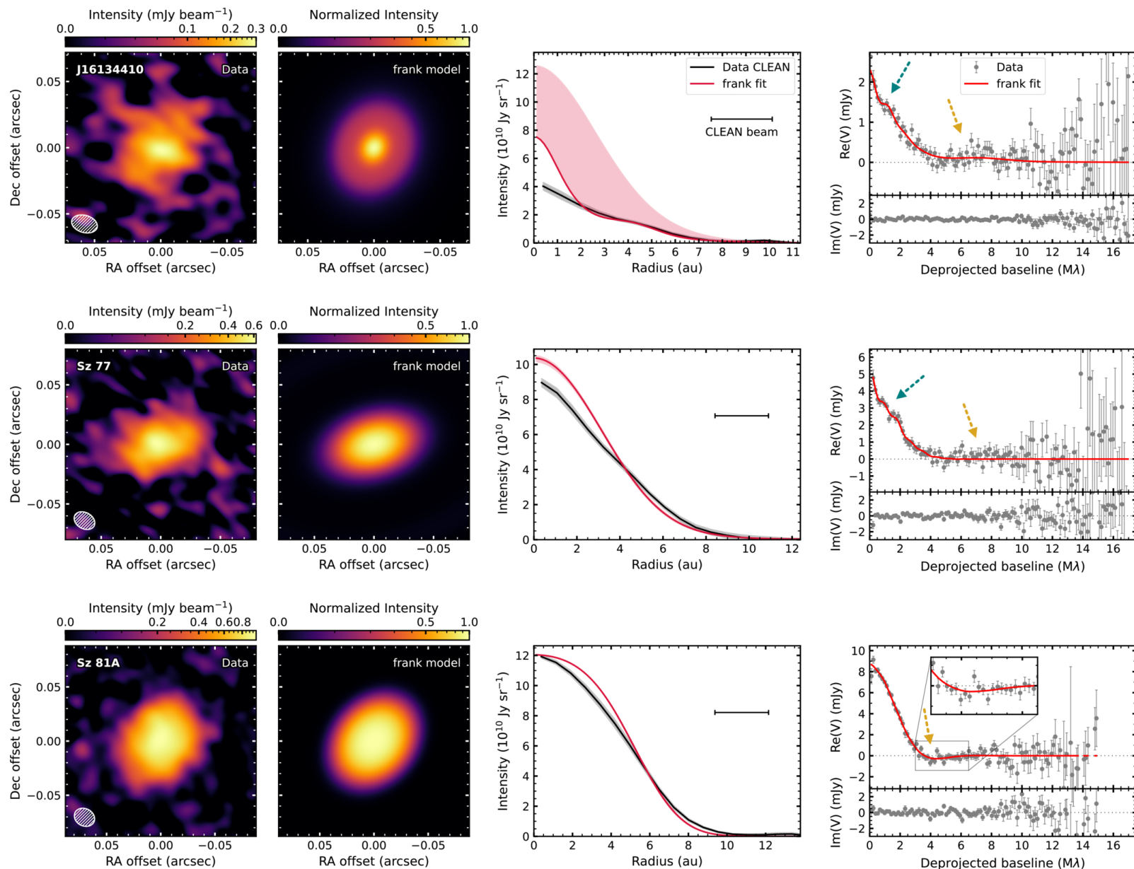
Figure 3. from Pietro Curone et al 2026 Astrophys. J. Lett. 1010 doi:10.3847/2041-8213/aeaa3c https://dx.doi.org/10.3847/2041-8213/aeaa3c © 2026. The Author(s). Published by the American Astronomical Society.
