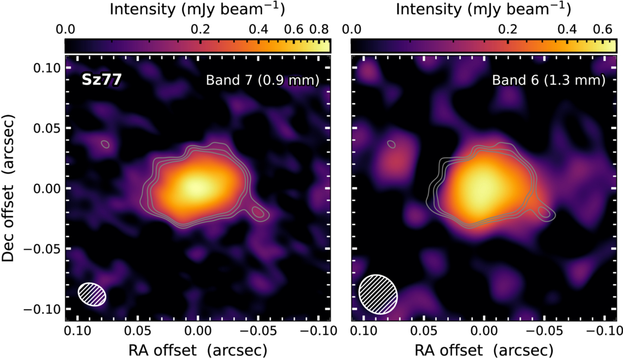
Figure A4. from Pietro Curone et al 2026 Astrophys. J. Lett. 1010 doi:10.3847/2041-8213/aeaa3c https://dx.doi.org/10.3847/2041-8213/aeaa3c © 2026. The Author(s). Published by the American Astronomical Society.
