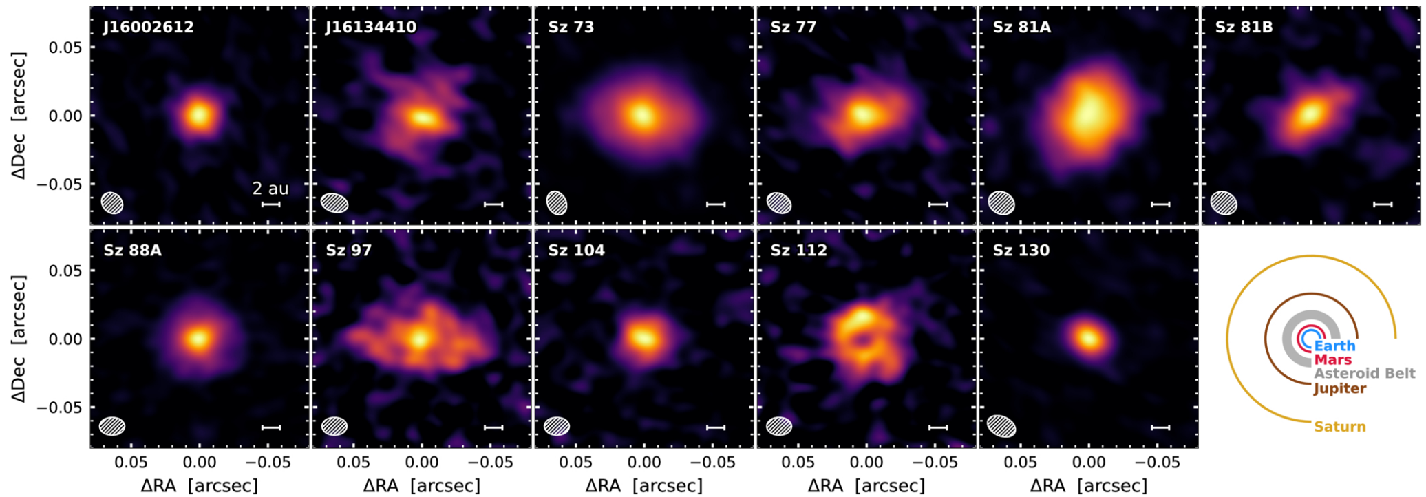
Figure 1. from Pietro Curone et al 2026 Astrophys. J. Lett. 1010 doi:10.3847/2041-8213/aeaa3c https://dx.doi.org/10.3847/2041-8213/aeaa3c © 2026. The Author(s). Published by the American Astronomical Society.
