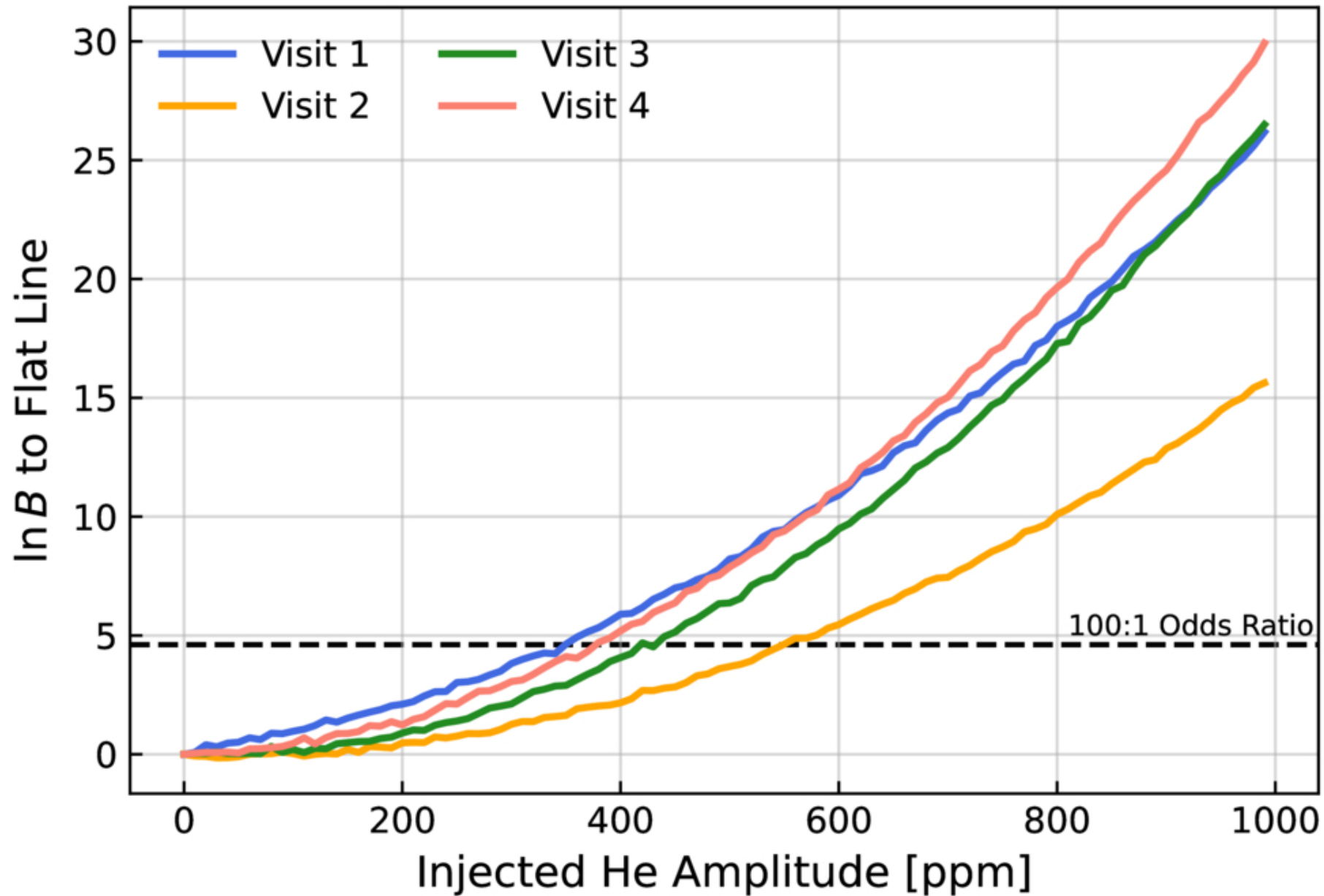
Figure 3. from Michael Radica 2026 Astrophys. J. Lett. 1010 doi:10.3847/2041-8213/aeaa39 https://dx.doi.org/10.3847/2041-8213/aeaa39 © 2026. The Author(s). Published by the American Astronomical Society.
