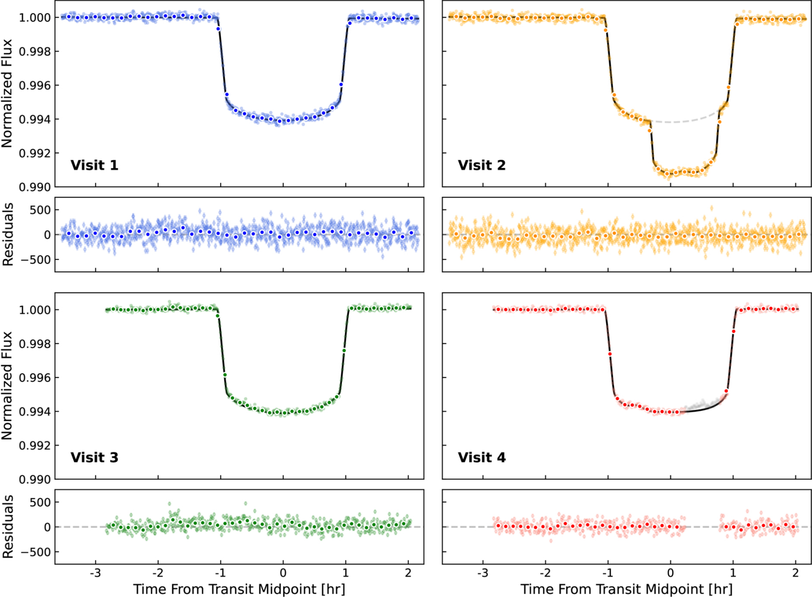
Figure 1. from Michael Radica 2026 Astrophys. J. Lett. 1010 doi:10.3847/2041-8213/aeaa39 https://dx.doi.org/10.3847/2041-8213/aeaa39 © 2026. The Author(s). Published by the American Astronomical Society.
