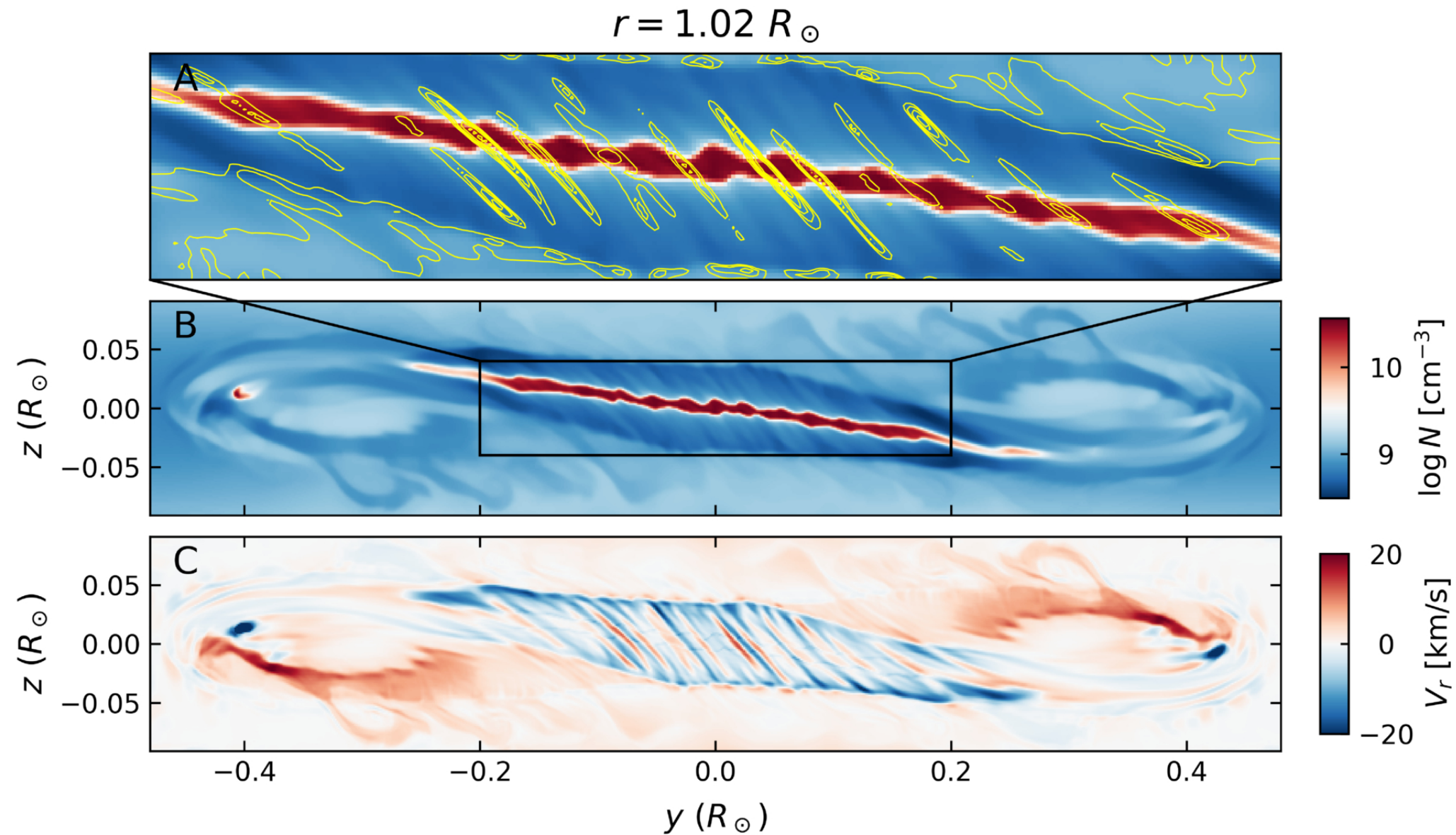
Figure 4. from Hongyang Luo and Yuhong Fan 2026 Astrophys. J. Lett. 1010 doi:10.3847/2041-8213/aeaa2e https://dx.doi.org/10.3847/2041-8213/aeaa2e © 2026. The Author(s). Published by the American Astronomical Society.
