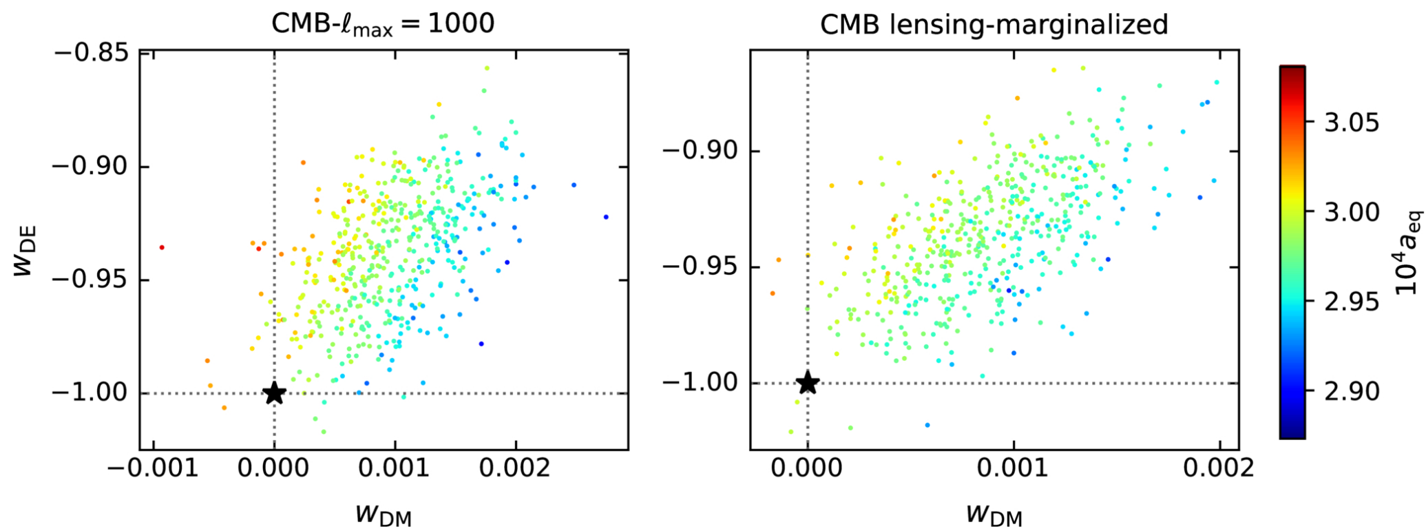
Figure 2. from Jun-Qian Jiang and Arman Shafieloo 2026 Astrophys. J. Lett. 1010 doi:10.3847/2041-8213/aeaa2a https://dx.doi.org/10.3847/2041-8213/aeaa2a © 2026. The Author(s). Published by the American Astronomical Society.
