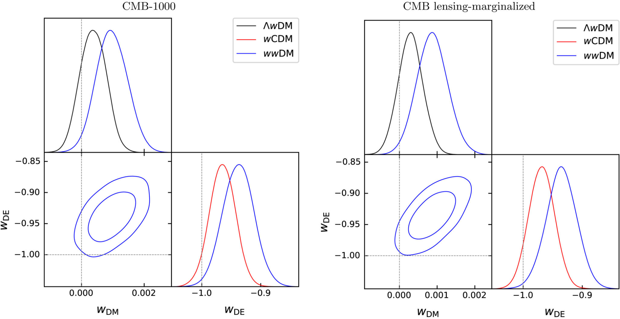
Figure 1. from Jun-Qian Jiang and Arman Shafieloo 2026 Astrophys. J. Lett. 1010 doi:10.3847/2041-8213/aeaa2a https://dx.doi.org/10.3847/2041-8213/aeaa2a © 2026. The Author(s). Published by the American Astronomical Society.
