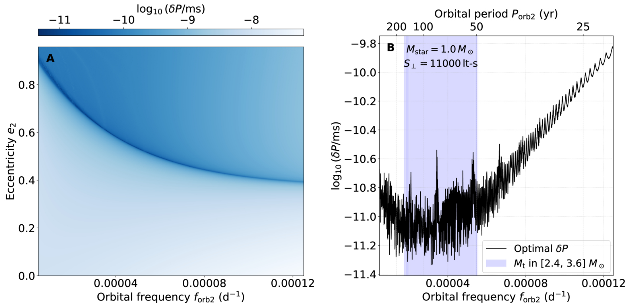
Figure 5. from Z. L. Yang et al 2026 Astrophys. J. Lett. 1010 doi:10.3847/2041-8213/aeaa29 https://dx.doi.org/10.3847/2041-8213/aeaa29 © 2026. The Author(s). Published by the American Astronomical Society.
