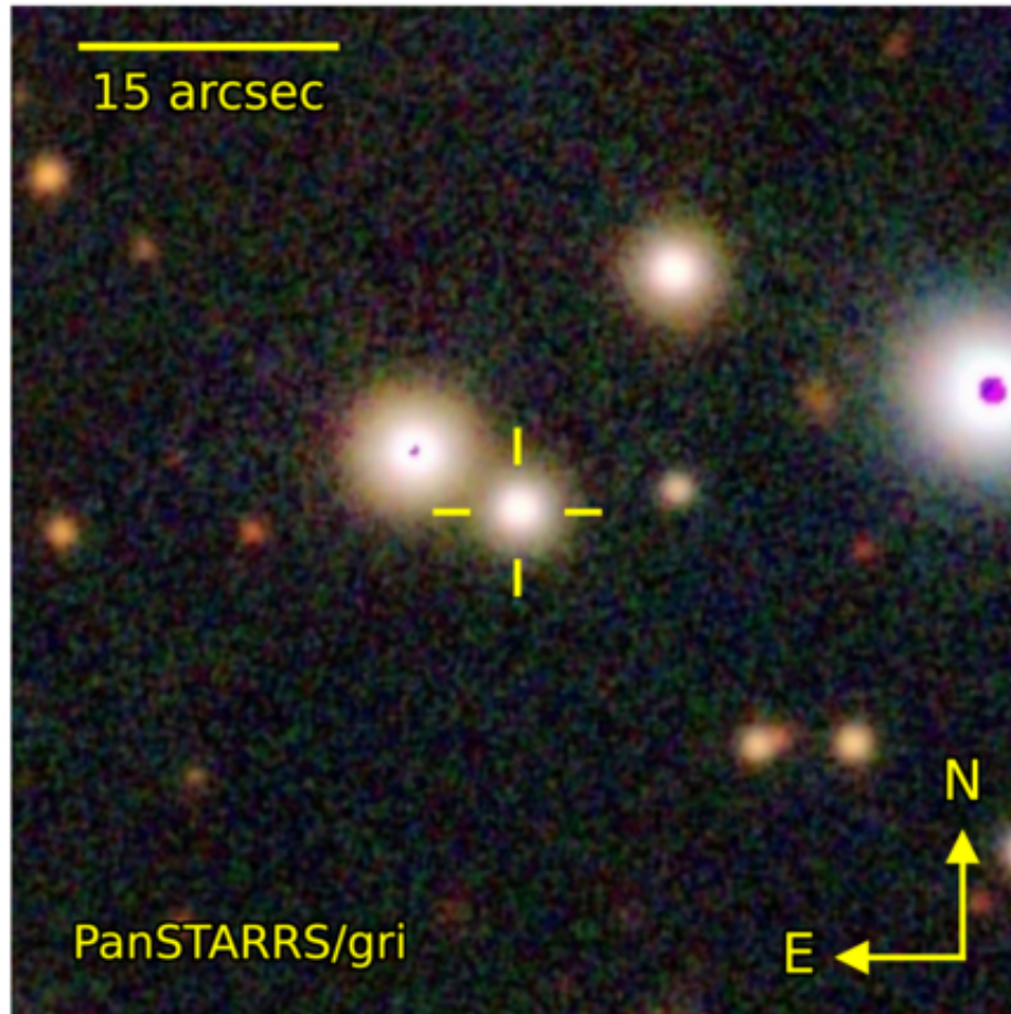
Figure 3. from Z. L. Yang et al 2026 Astrophys. J. Lett. 1010 doi:10.3847/2041-8213/aeaa29 https://dx.doi.org/10.3847/2041-8213/aeaa29 © 2026. The Author(s). Published by the American Astronomical Society.
