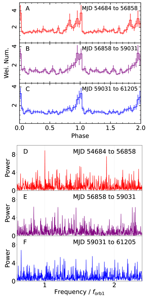
Figure 10. from Z. L. Yang et al 2026 Astrophys. J. Lett. 1010 doi:10.3847/2041-8213/aeaa29 https://dx.doi.org/10.3847/2041-8213/aeaa29 © 2026. The Author(s). Published by the American Astronomical Society.
