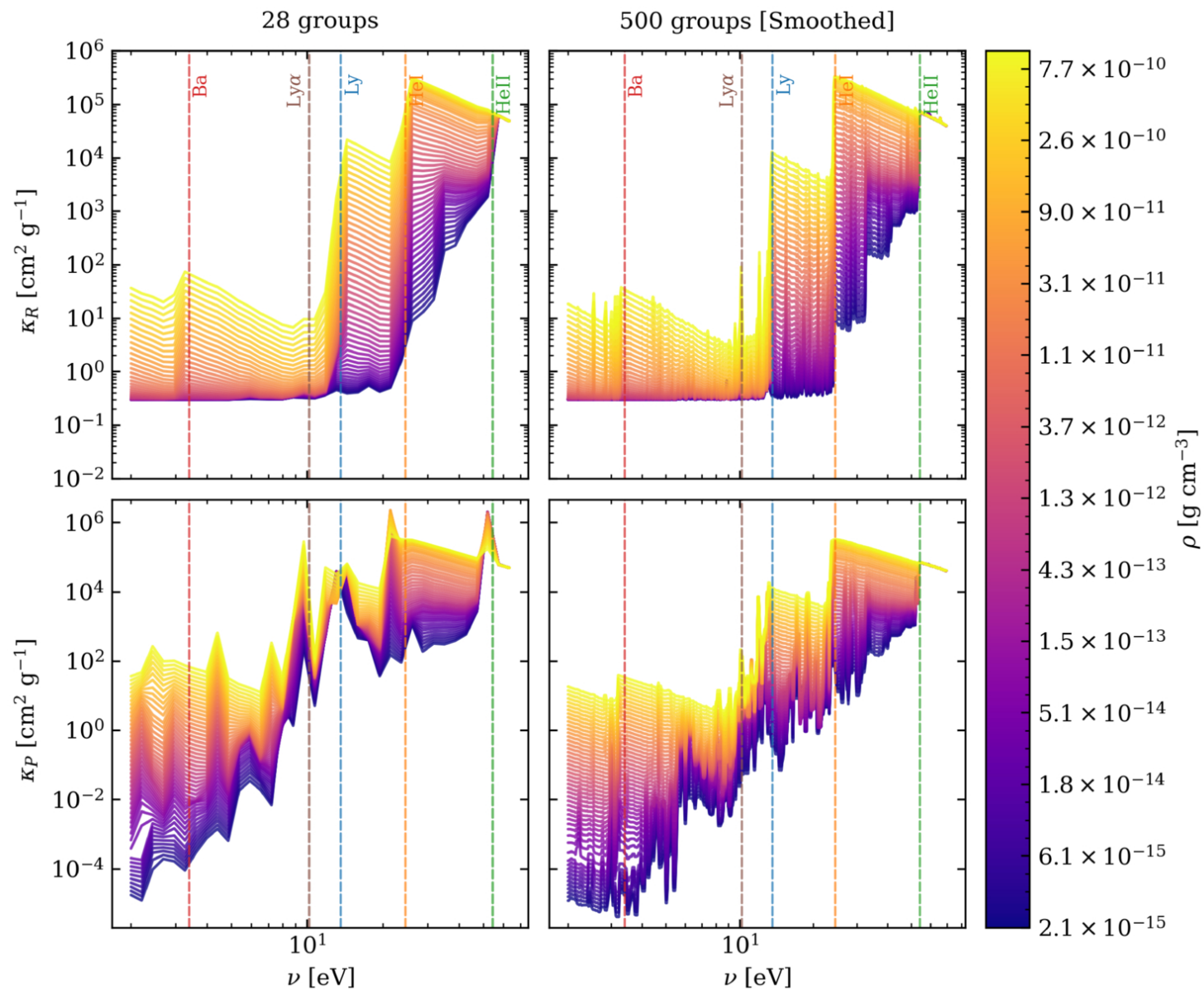
Figure A1. from Ish Kaul et al 2026 Astrophys. J. Lett. 1009 doi:10.3847/2041-8213/aea981 https://dx.doi.org/10.3847/2041-8213/aea981 © 2026. The Author(s). Published by the American Astronomical Society.
