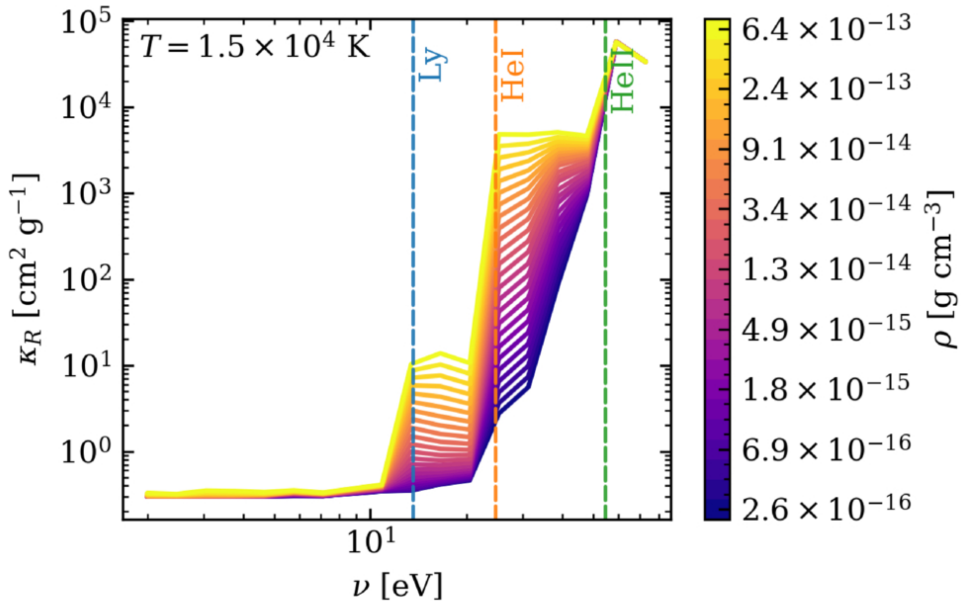
Figure 6. from Ish Kaul et al 2026 Astrophys. J. Lett. 1009 doi:10.3847/2041-8213/aea981 https://dx.doi.org/10.3847/2041-8213/aea981 © 2026. The Author(s). Published by the American Astronomical Society.
