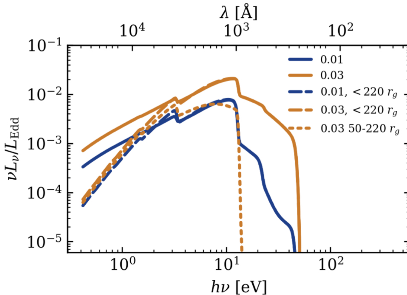
Figure 4. from Ish Kaul et al 2026 Astrophys. J. Lett. 1009 doi:10.3847/2041-8213/aea981 https://dx.doi.org/10.3847/2041-8213/aea981 © 2026. The Author(s). Published by the American Astronomical Society.
